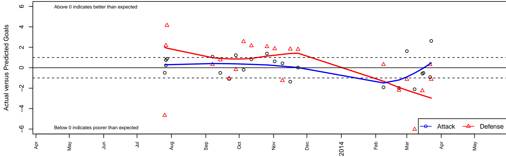
Seattle Celtic Orange B02 Dots are actual minus expected GF (blue circles) and GA (red triangles). Blue line is smoothed change in attack strength. Red is smoothed change in defense strength.
